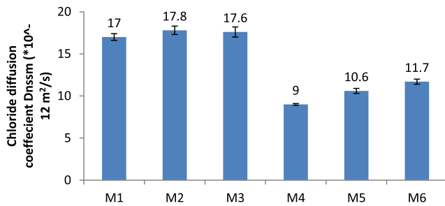
Fig. 5. Chloride diffusion rates of the AAC mixes tested.
