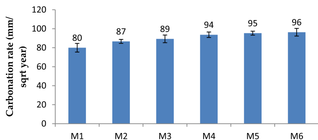
Fig. 6. Accelerated carbonation rate of the AAC mixes tested.
