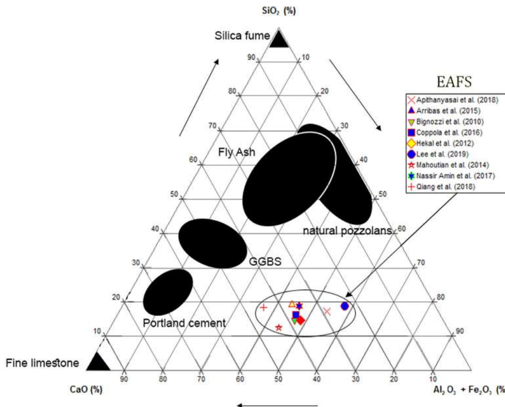
Fig. 1. Ternary diagram with the chemical composition of possible precursors for AAC (adapted from Lothenbach et al. [13]).
