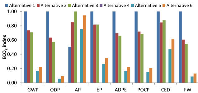
Fig. 9. Normalized environmental impact indicators for plain concrete scenario.
