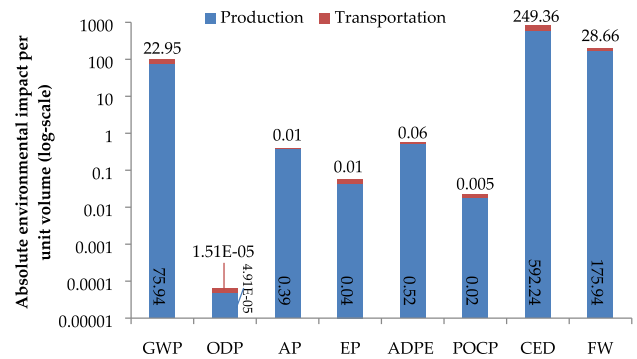
Fig. 7. Contribution of transportation processes to the total environmental impact of alternative 1.
