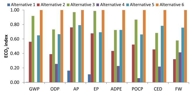
Fig. 8. Normalized environmental impact indicators for plain concrete scenario.
