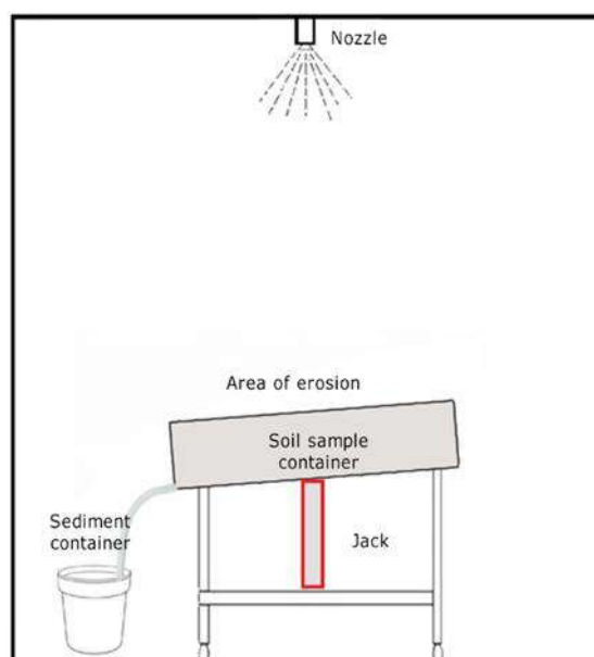
Figure 2. Cross-section view of the rainfall simulator (20).
