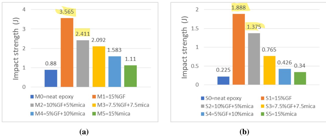
Figure 8 (a) The result of impact strength composite materials master brace. (b) The result of impact strength composite materials sikadur.
