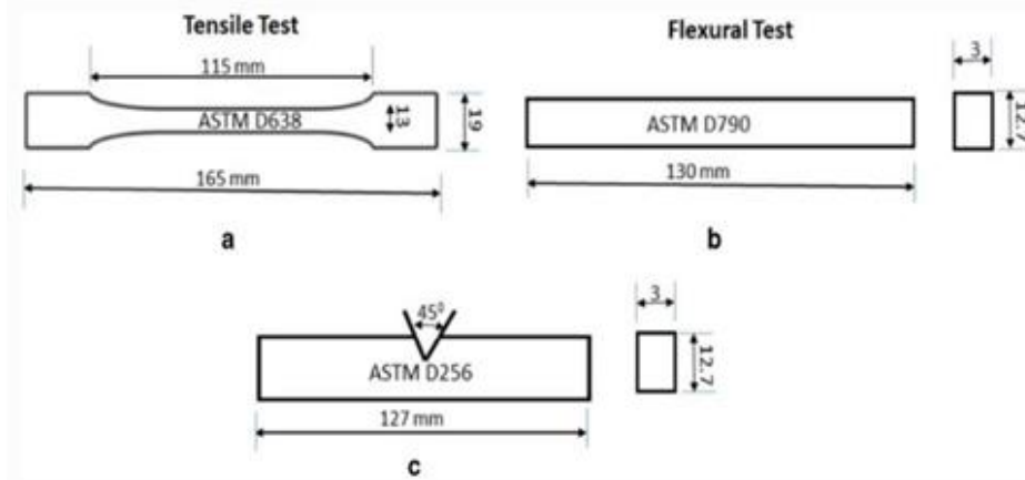
Figure 4 (a) ASTM D638 standard for tensile samples. (b) ASTM D790 standard for flexural samples. (c) ASTM D256 standard for impact charpy samples.
