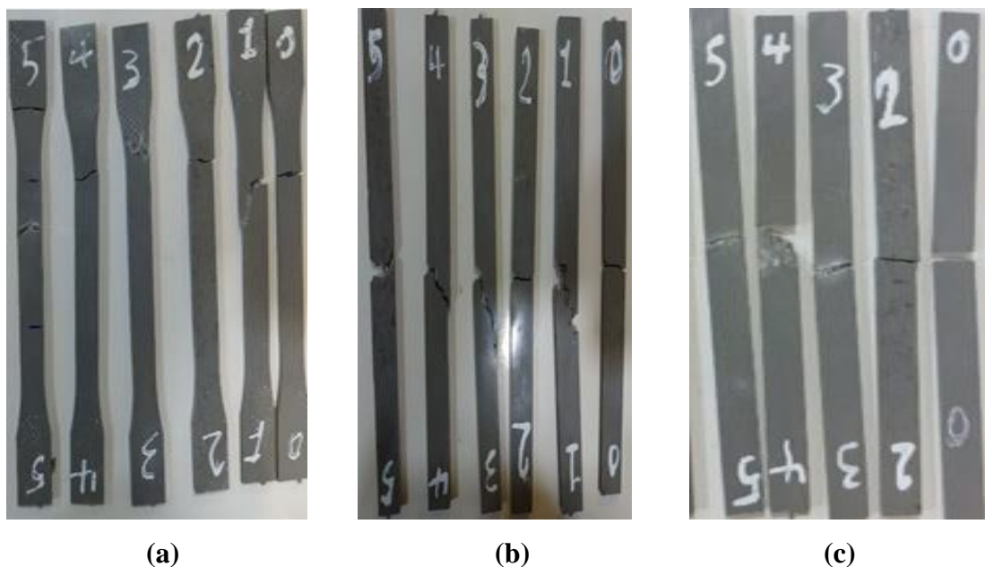
Figure 5 (a) Tensile samples after testing, (b) Impact samples after testing, (c) Flexural samples after testing.
