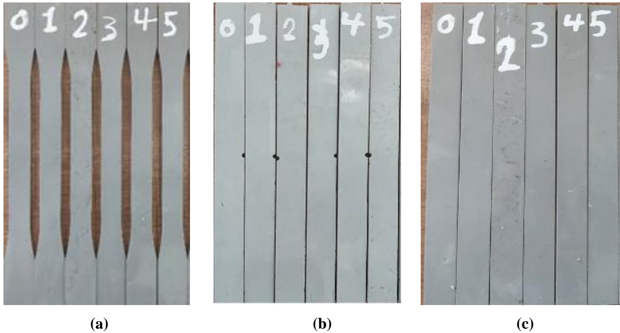
Figure 3 (a) Tensile test samples, (b) Impact test samples, (c) Flexural test samples.
