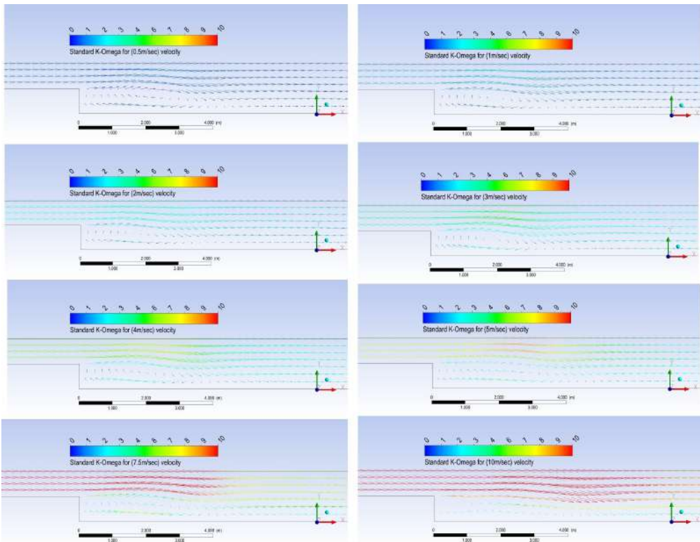
Fig. 4. Velocity vector with vortices for different values of Reynolds number for Wilcox K-\epsilon model
