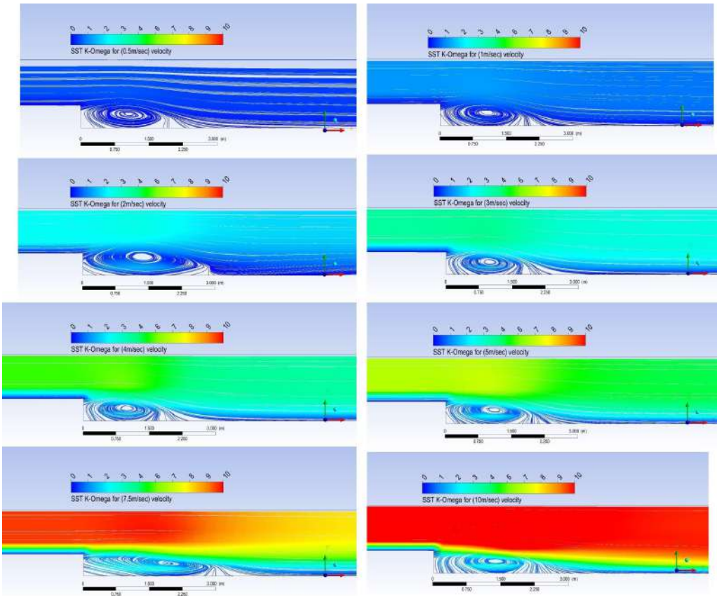
Fig. 3. Velocity contour for different values of velocity for SST K- \omega model
