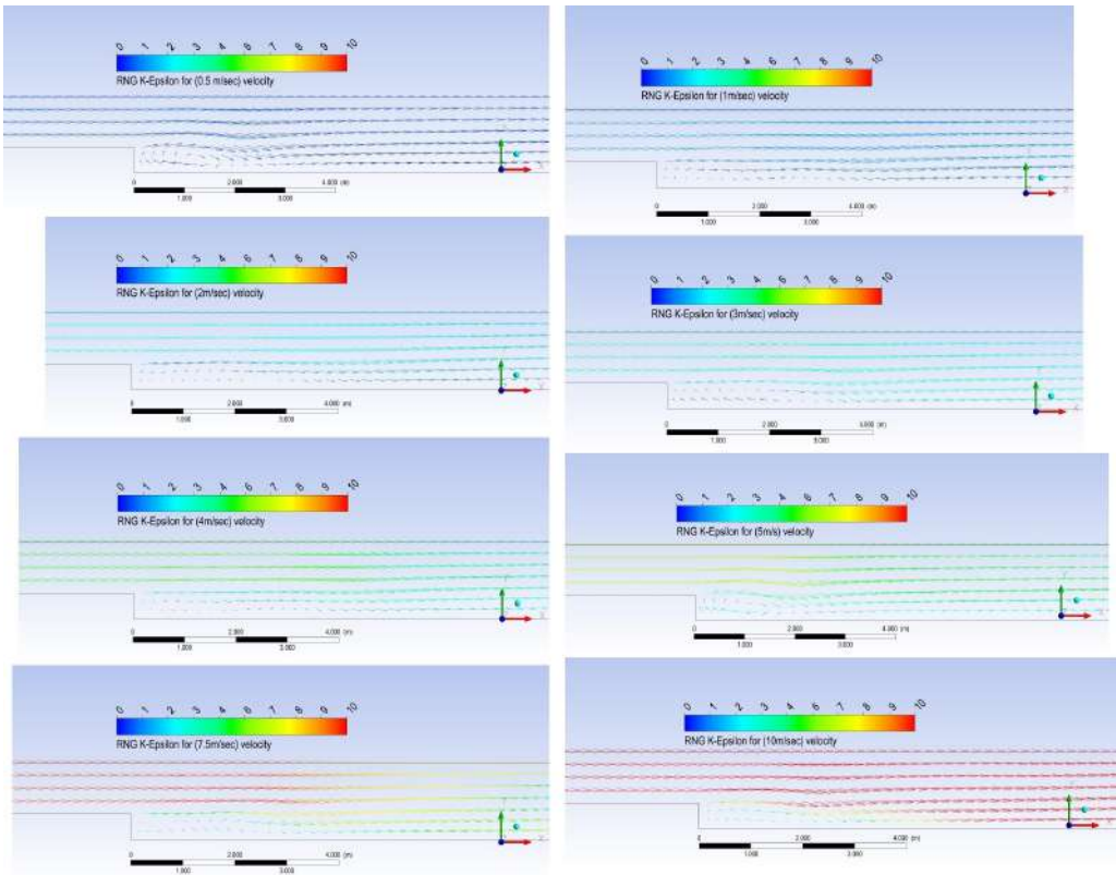
Fig. 2. Velocity vector with vortices for different values of Reynolds number for RNG K- \epsilon model
