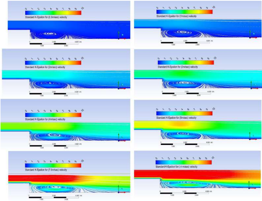
Fig. 5. Velocity contour for different values of velocity for standard K- \epsilon model
