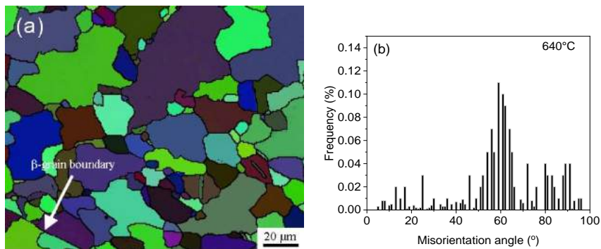
Fig. 8 640B aging sample (a) IPF-EBSD image (b) MAD histogram
