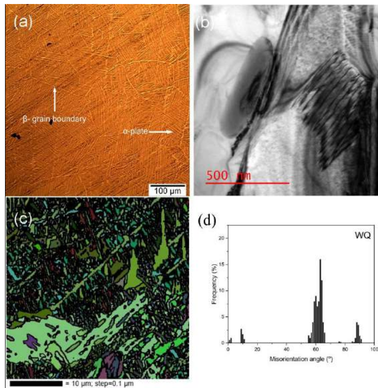
Fig. 2 \beta -quenching microstructure: (a) optical micrograph (b) BF-TEM image (c) EBSD-IPF Image (d) MAD histogram
