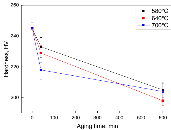
Fig. 9 Vickers micro-hardness results of \beta -quenching and aging samples
